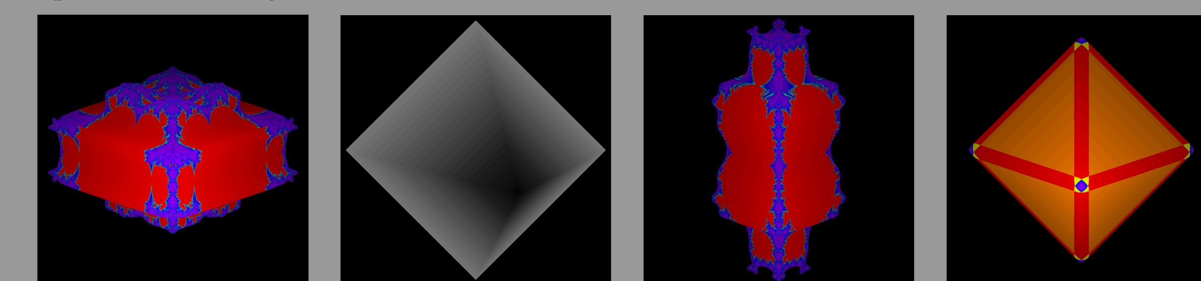
Fig. 6: Tetrabrot Fig. 7: Perplexbrot Fig. 8: Hourglassbrot Fig. 9: Metabrot
